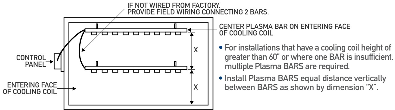
FIGURE 1c Plasma BAR Installation for Air Handlers Requiring Multiple BARS
