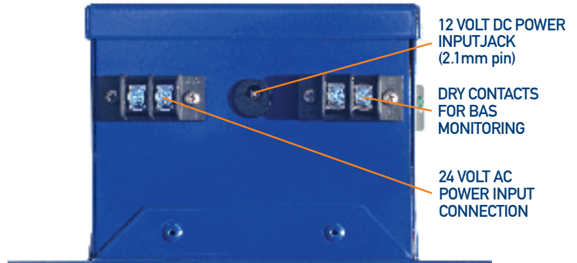
FIGURE 4 – Left view of PB-CP control panel
